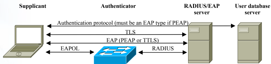
Figure 2: protocol layering in EAPs PEAP and TTLS.
